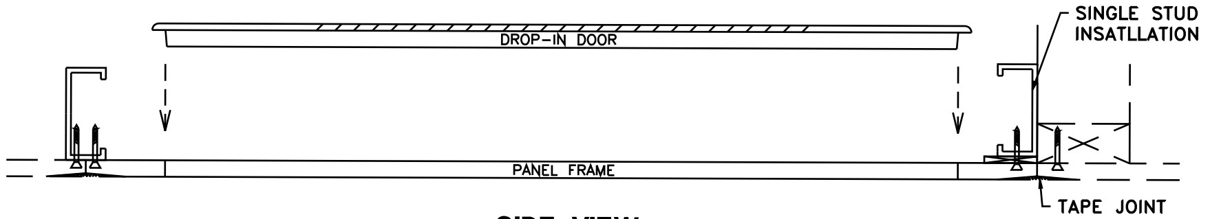
SIDE VIEW
