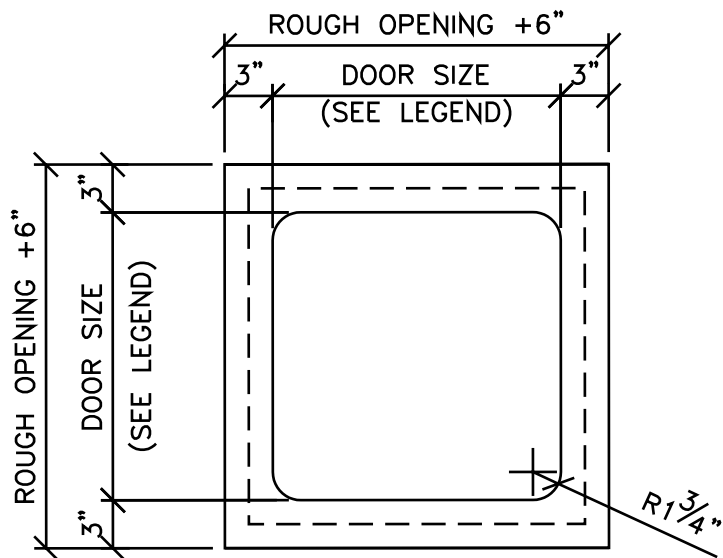
TYP. PANEL ELEVATION
