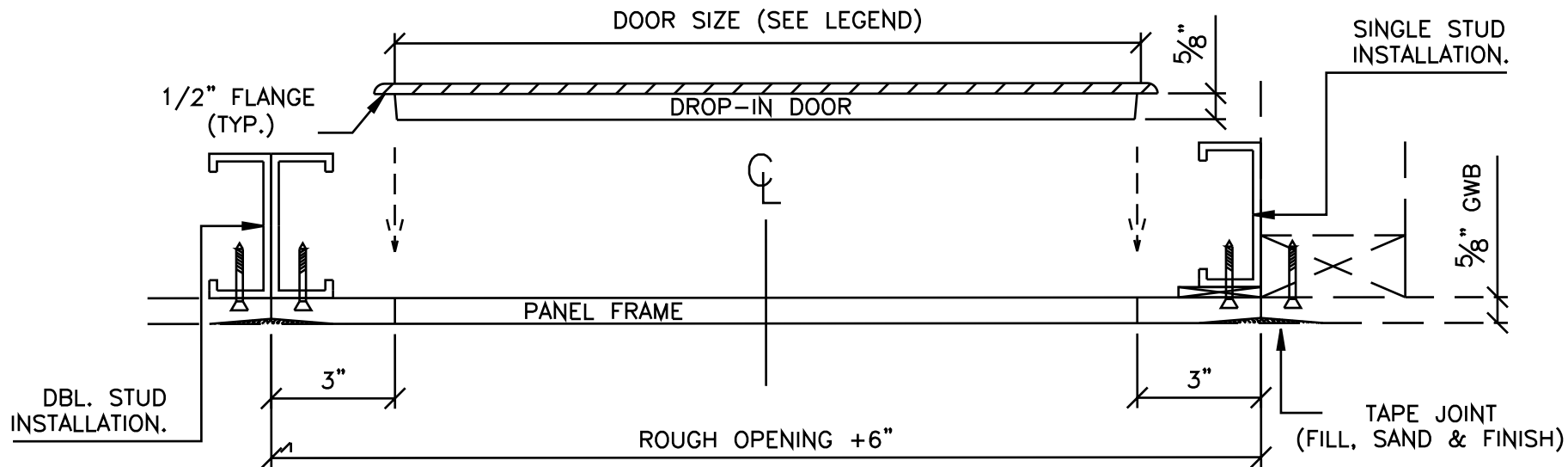
SIDE VIEW
